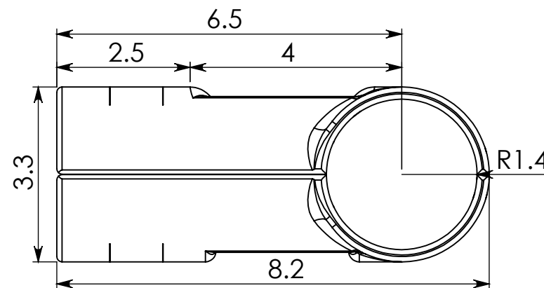
V lateral
